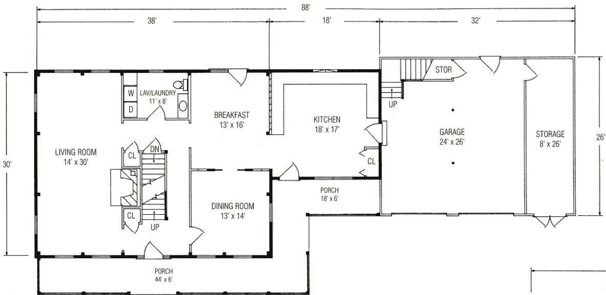
FIRST FLOOR 1,446 SQUARE FEET
