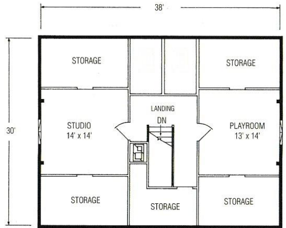
THIRD FLOOR 1,047 SQUARE FEET
