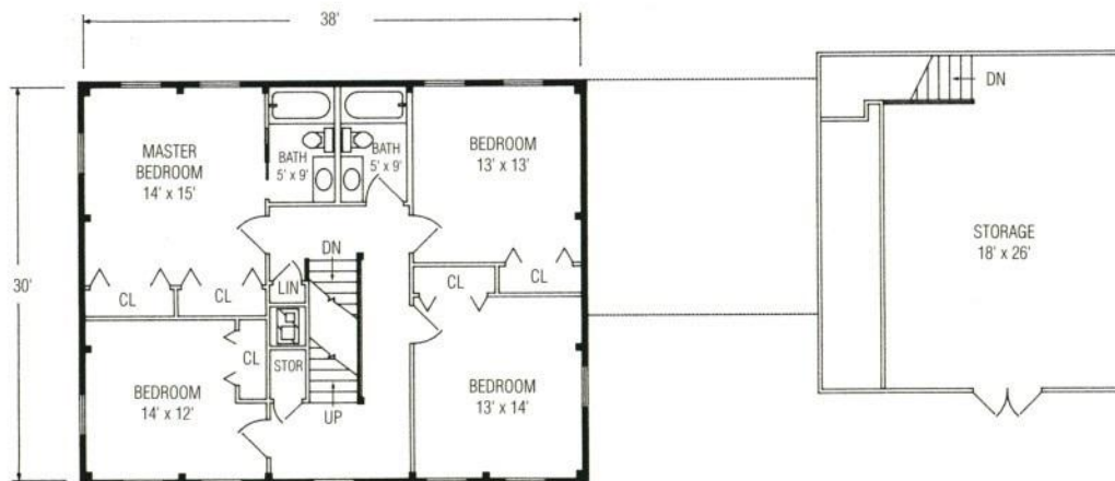
SECOND FLOOR 1,140 SQUARE FEET
