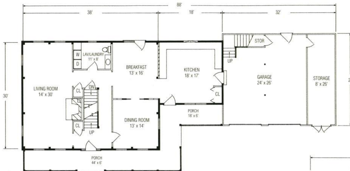
FIRST FLOOR 1,446 SQUARE FEET
