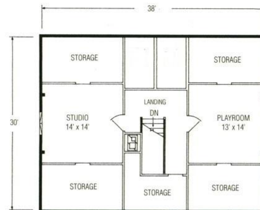
THIRD FLOOR 1,047 SQUARE FEET
